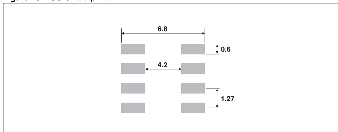
Figure 18. SO-8 Footprint
