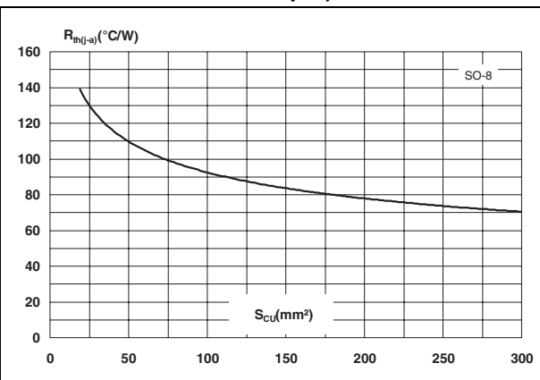
Figure 8. SO-8 junction to ambient thermal resistance versus copper surface area under tab (PCB FR4, copper thickness 35 \mu m)
